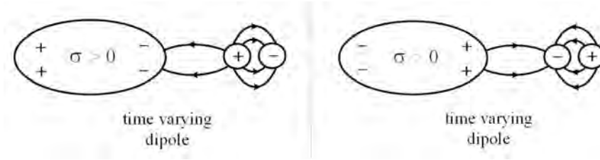
Figure 32.2: If the source that induces the charges on the conductor is time varying, the current in the conductor is always nonzero so that the charges can move around to respond to the external time-varying charges. The two figures above show the orientation of the charges for two snap-shot in time.
