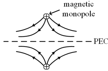
Figure 32.6: On a PEC surface, \hat{n} \cdot \mathbf{B} = 0 . Hence, a magnetic monopole on top of a PEC surface will have magnetic field distributed as shown.
