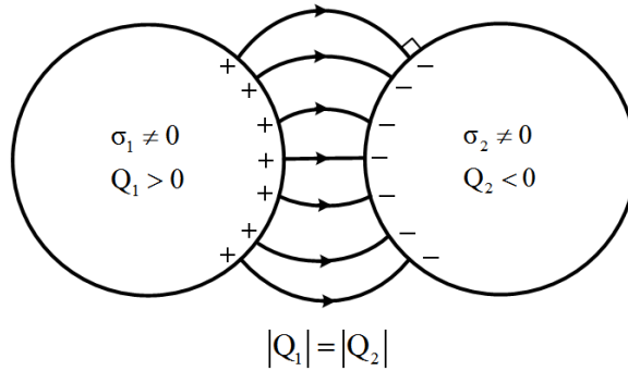
Figure 32.1: The objects can just be conductors, and in the quiescent state (static state), the tangential electric field will be zero on their surfaces.
