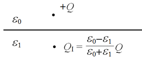
Figure 32.13: A static charge over a dielectric interface can be found in closed form.
