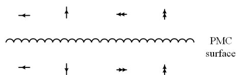
Figure 32.10: Reflection rules for electric and magnetic dipoles over a PMC surface.
