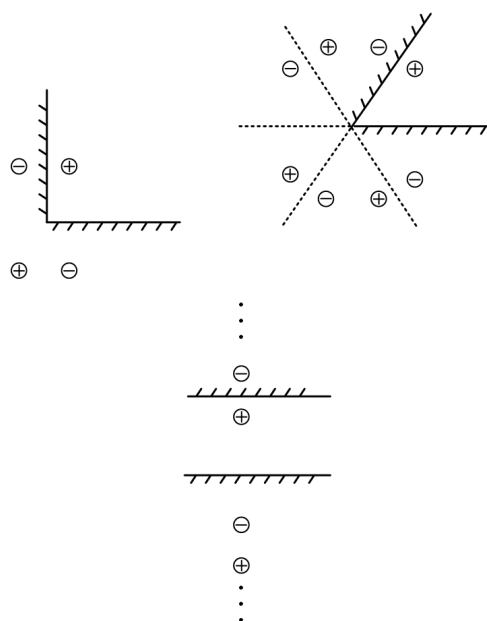
Figure 32.10: Reflection rules for electric and magnetic dipoles over a PMC surface.
