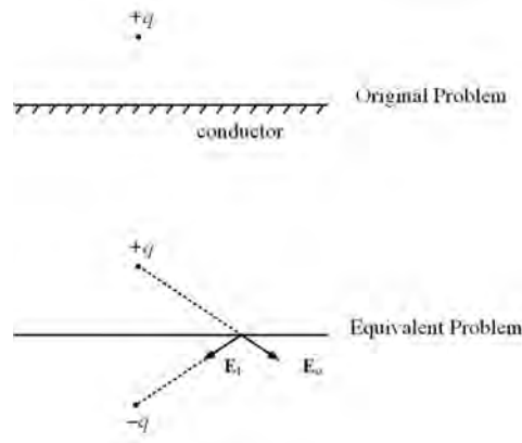
Figure 32.3: The use of image theory to solve the BVP of a point charge on top of a conductor. The boundary condition is that \hat{n} \times \mathbf{E} = 0 on the conductor surface.
